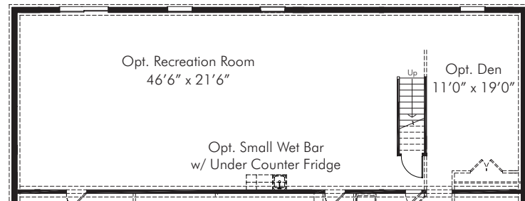
Optional Lower Level At Extended Great Room & Master Bedroom Elevation 1
