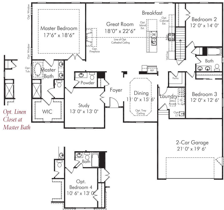
Optional Main Level At Optional Fourth Bedroom
